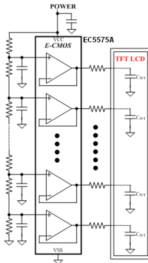
Figure 3. Typical Application Configuration.
