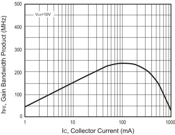
Fig.7 Gain Bandwidth Product vs. Collector Current
