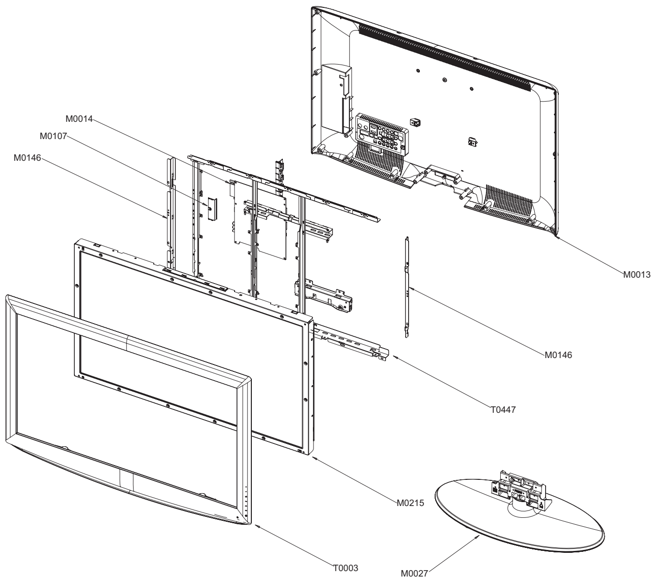
5-13 LE40R86BDX/LE40R86BCX Exploded View
